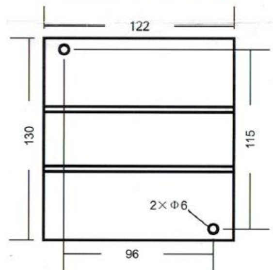
Installation Dimensions(mm)
